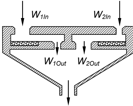
Figure 2. Schematic of sampler comprising two inertial impactors arranged in parallel.
